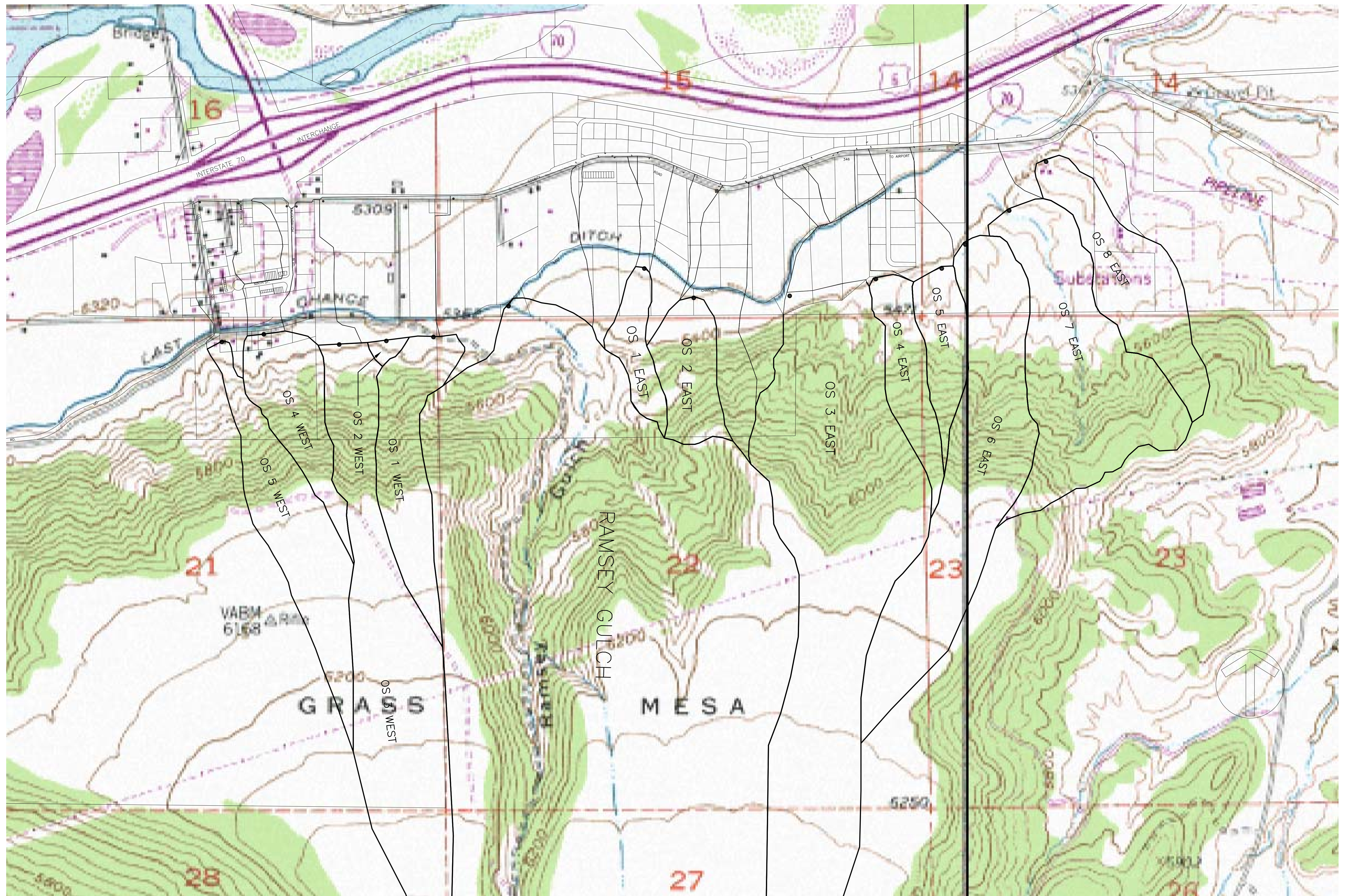
Figure 3-2 Offsite Basins Expanded View
