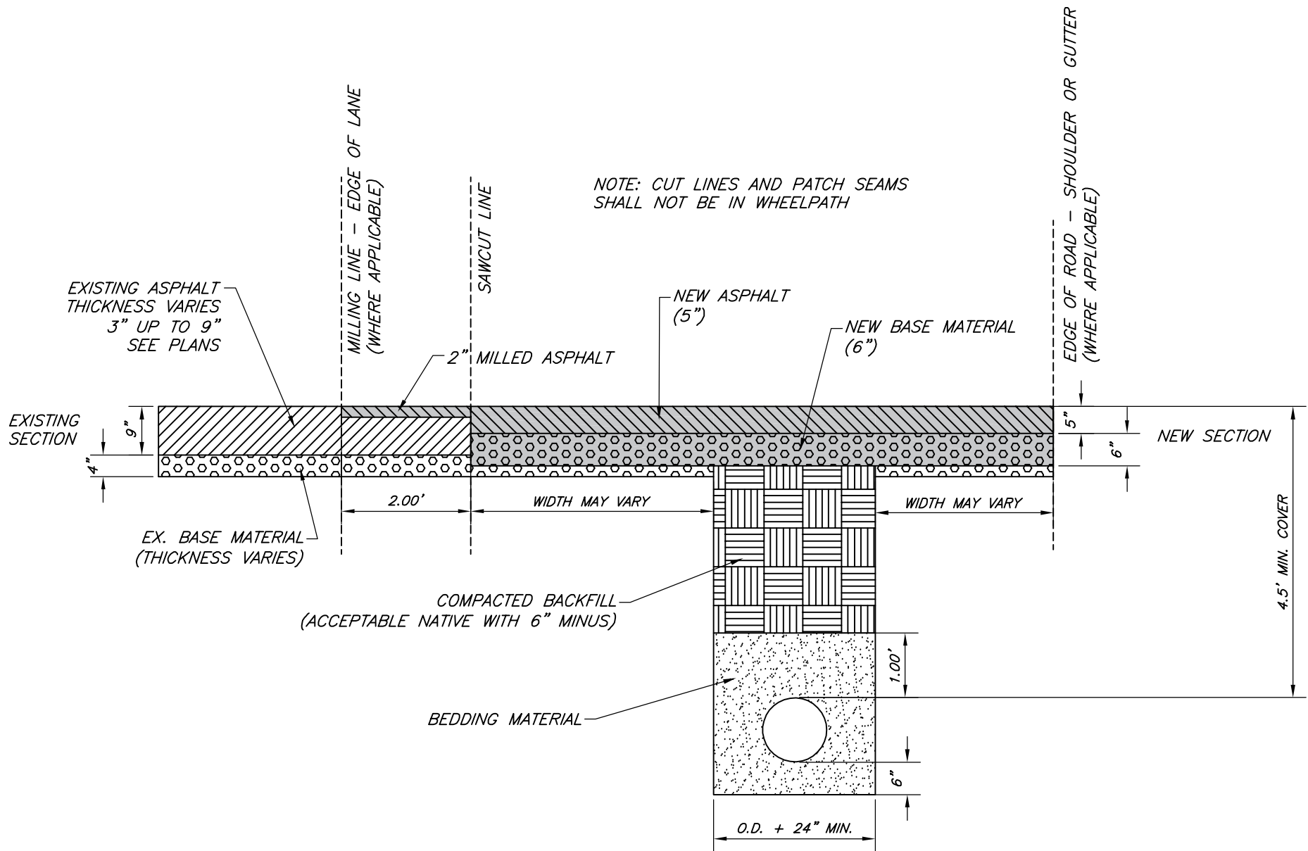
ASPHALT PATCH DETAIL
